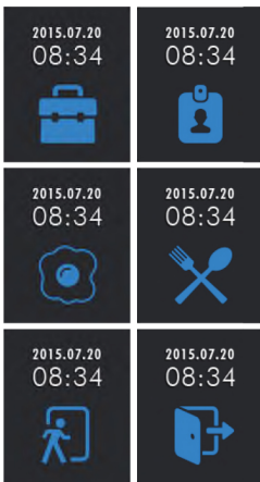
[Intuitive GUI]
